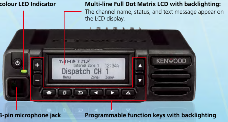
7-colour LED Indicator
